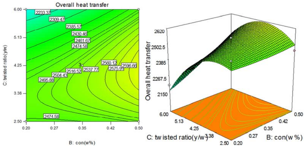
Figure 7. Response surface plots for the effect of the concentration(w%) and twisted ratio(y/w) on the overall heat transfer coefficients.
